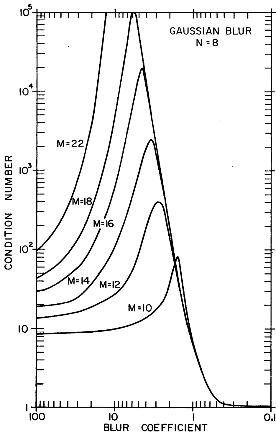
Figure (5.1-16) Blur Coefficient, Condition Number Curves for Gaussian Blur and Different Number of Sampled Values
