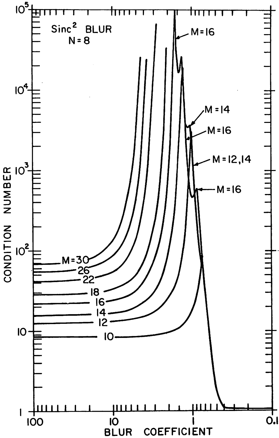
Figure (5.1-17) Blur Coefficient, Condition Number Curves for Sinc 2 Blur and Different Number of Sampled Values
