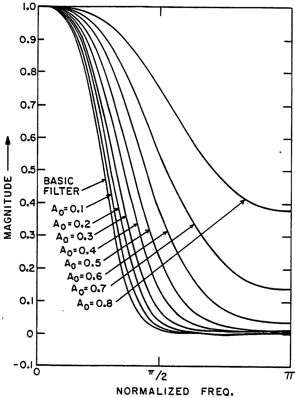
Figure 6-3. First-order transformation examples
