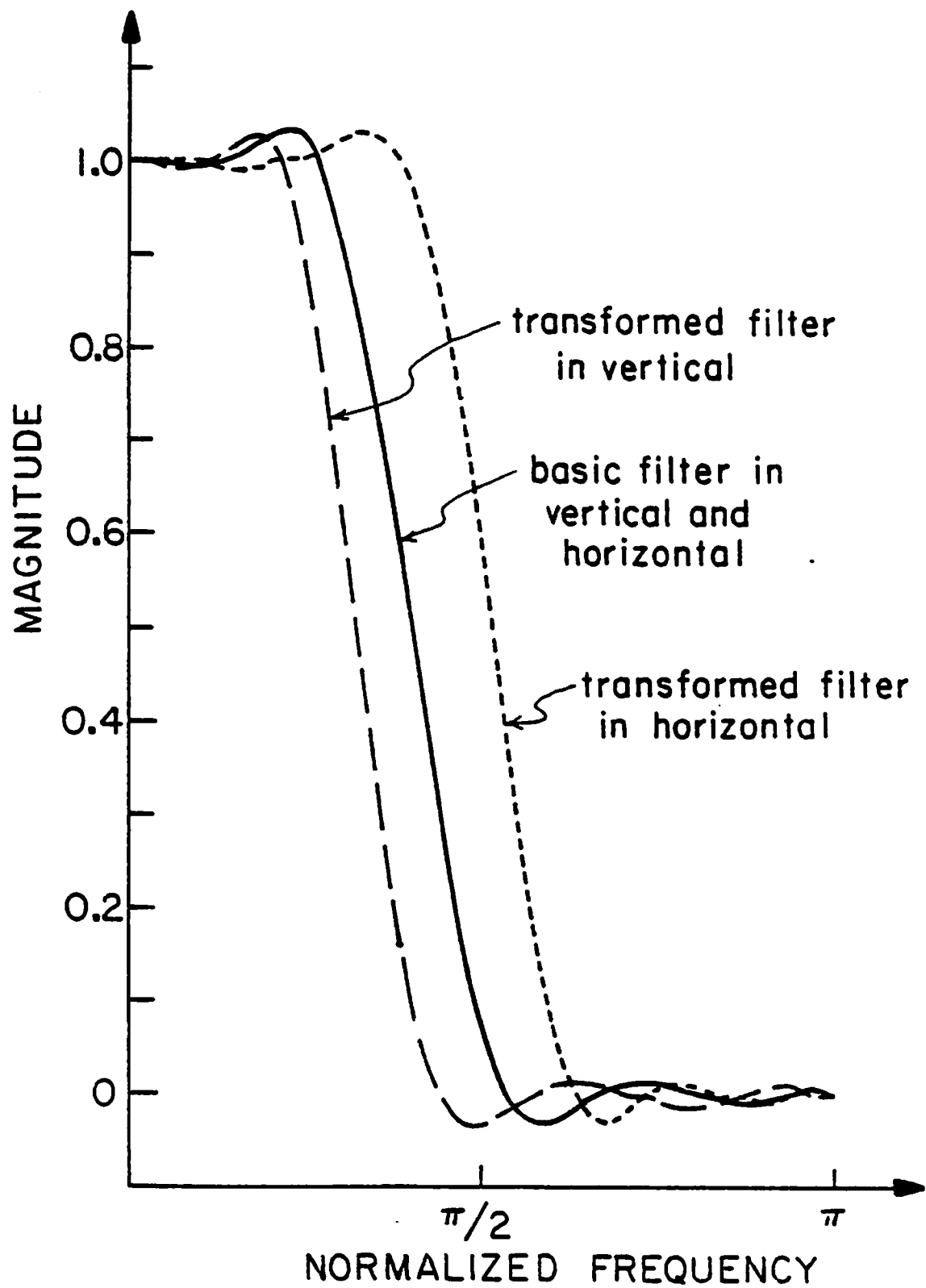
Figure 6-13. Second-order transformation for \beta_{c_1} \neq \beta_{c_2} (horizontal)
