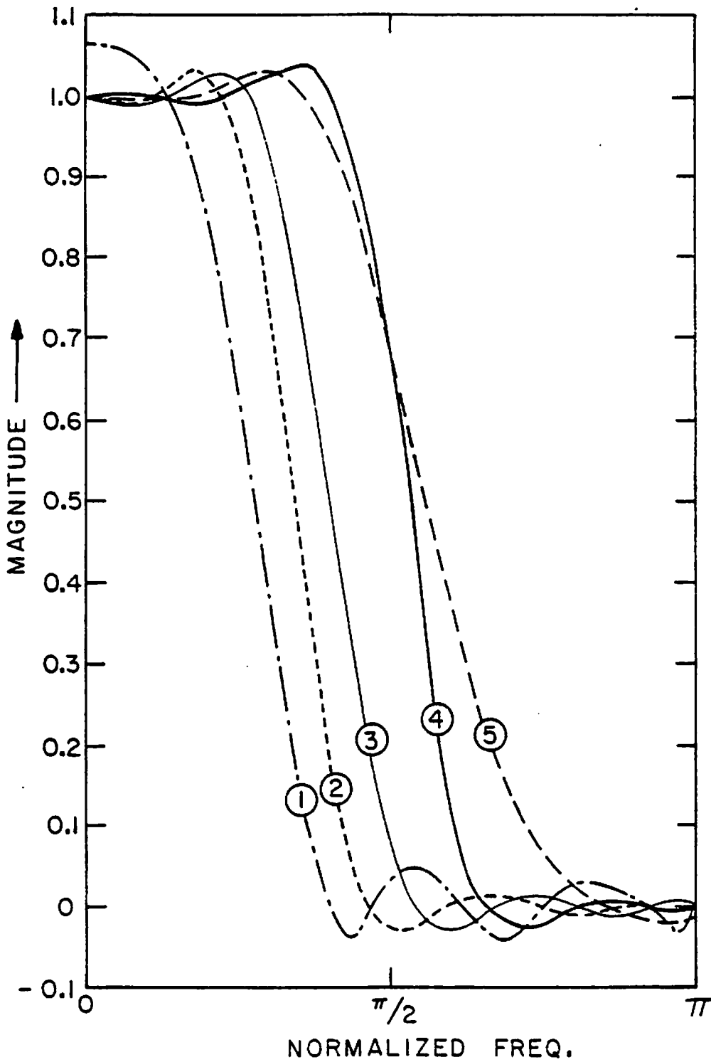
Figure 6-11. Transformation on the SVD/SGK convolution filter (horizontal)
