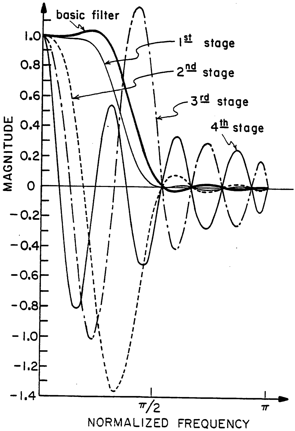
Figure 6-7. SVD-expanded filter frequency response 147
