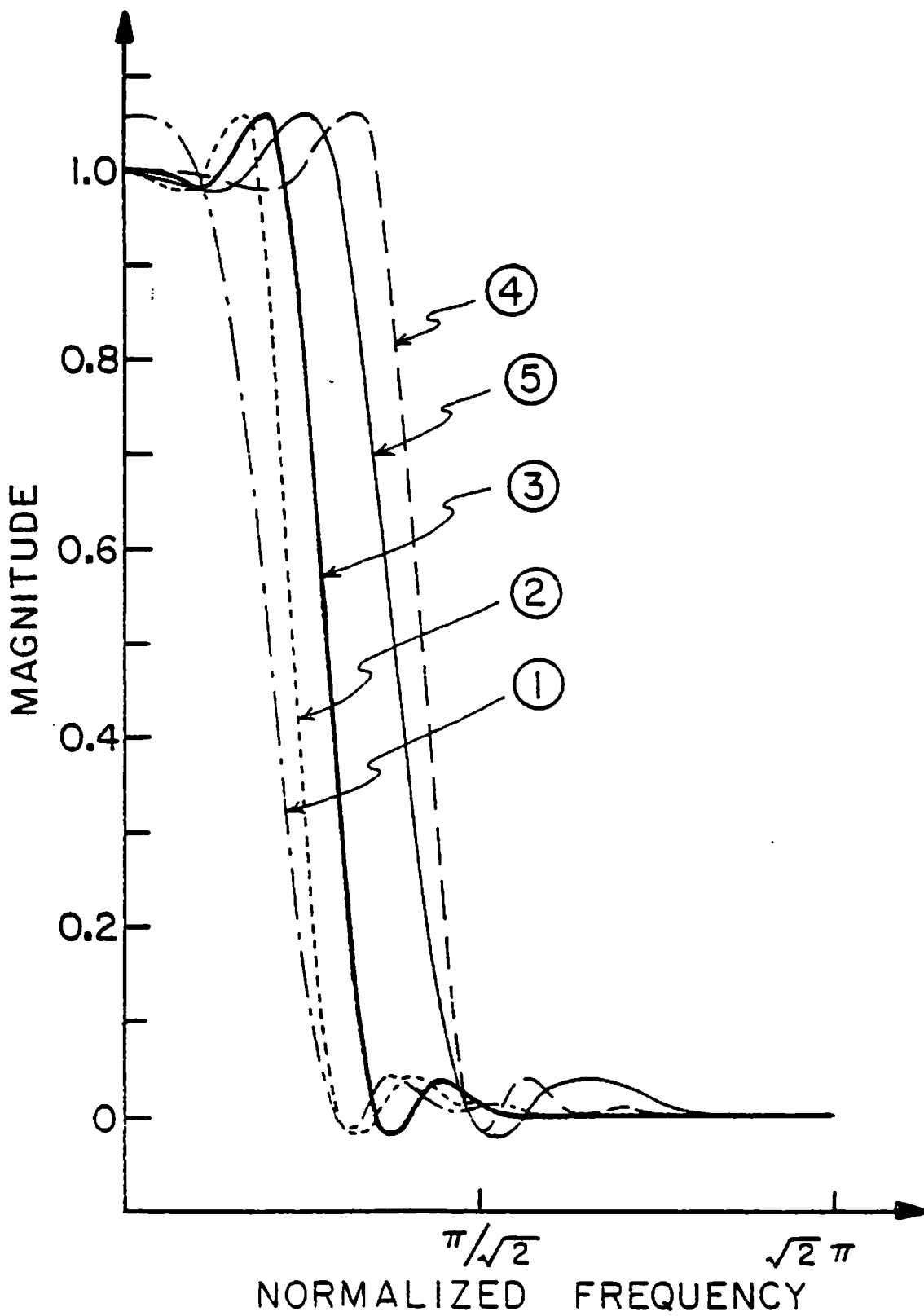
Figure 6-12. Transformation on the SVD/SGK convolution filter (diagonal)
