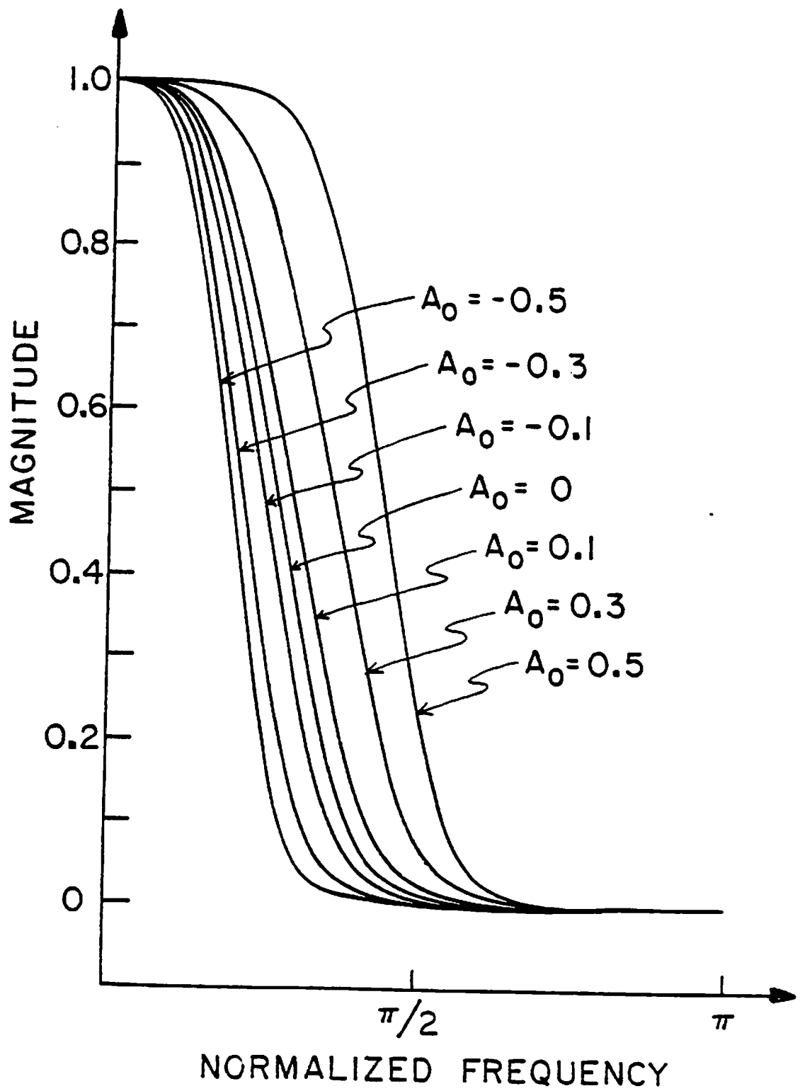
Figure 6-5. Second-order transformation examples
