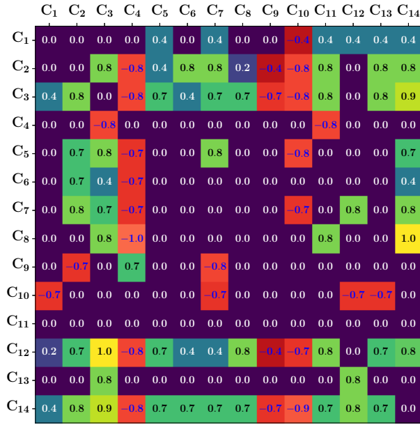
(c) Reconstructed edges E_2 from latent II.
