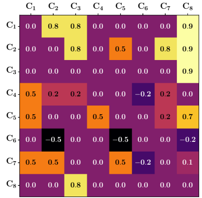
(c) Reconstructed edges latent II: E_2
