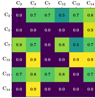
(b) Reconstructed edges from latent I: E_1
