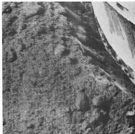
b) Inverse Fourier Transform of Fourier Transform
