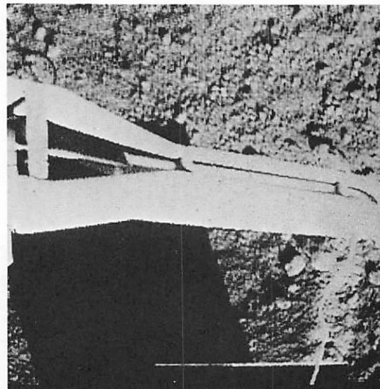
b) Inverse Fourier Transform of Fourier Transform
