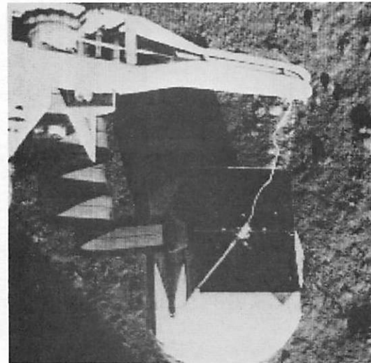
d) Inverse Fourier Transform of Gaussianly Quantized Fourier Transform of box, p = 500
