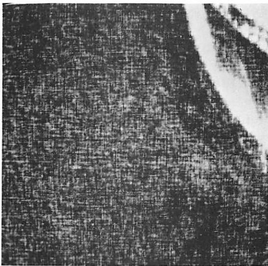
c) Reconstruction with the 800 Lowest Spatial Frequencies Errorless
