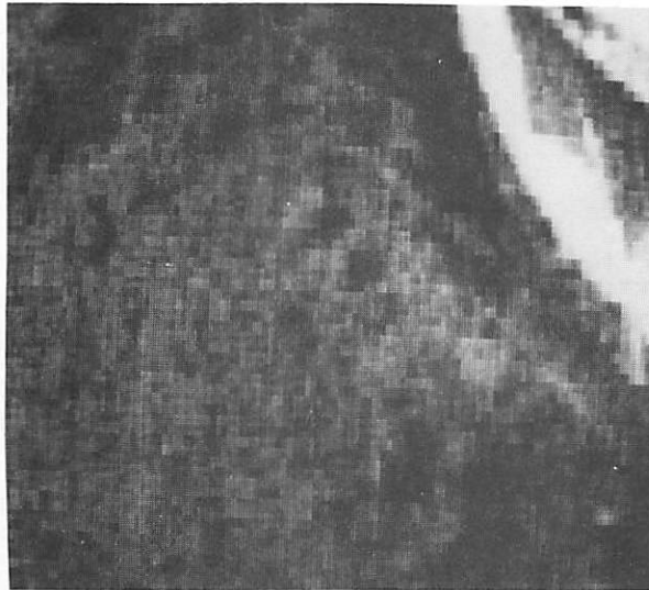
Figure 5-6. Low Pass Zonal Hadamard Transform Sampling - Footpad
