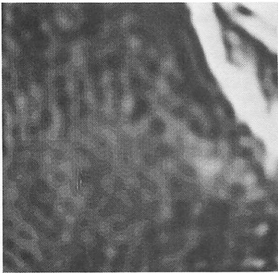
a) 99.8% energy transmitted, 32:1 BWR
