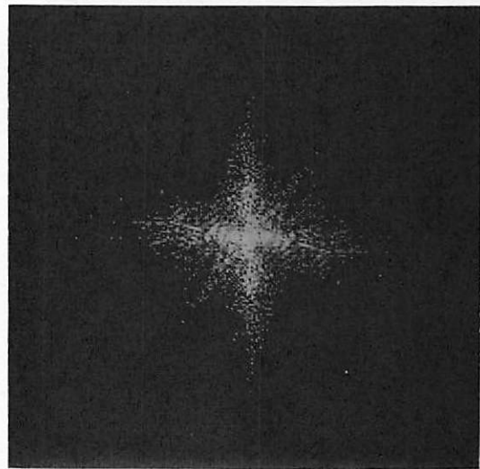
d) Logarithm of Magnitude of Fourier Transform
