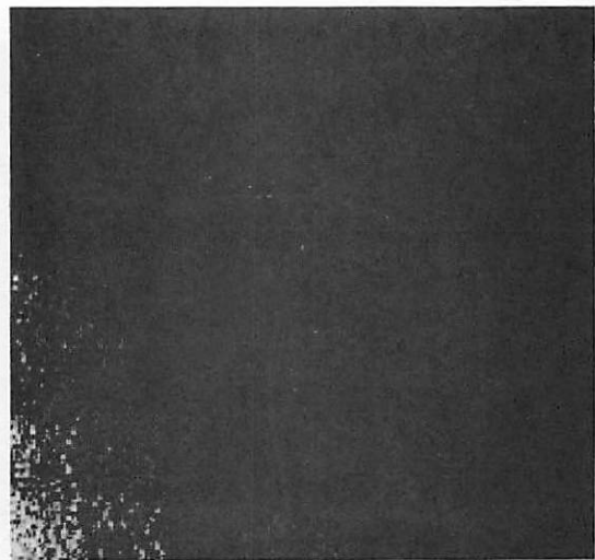
d) Logarithm of Magnitude of Hadamard Transform
