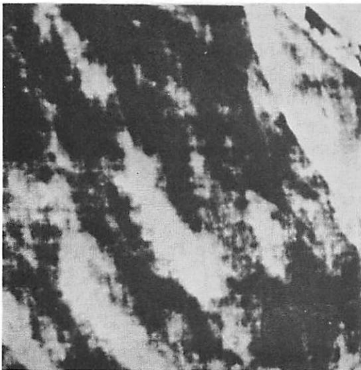
b) Random Sampling
