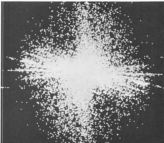
c) Map of Samples Above 200
