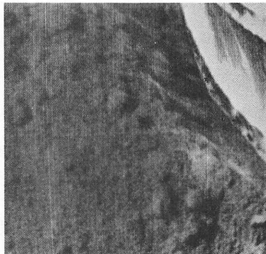
b) Inverse Fourier Transform of Gaussianly Quantized Fourier Transform with a Wide Gaussian Shaped Variance Function, p = 1000
