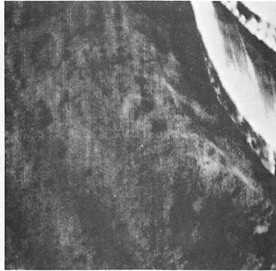
a) Inverse Fourier Transform of Gaussianly Quantized Fourier Transform - 32 levels
