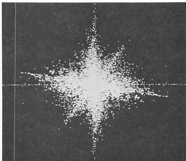
a) Map of Samples Above 300
