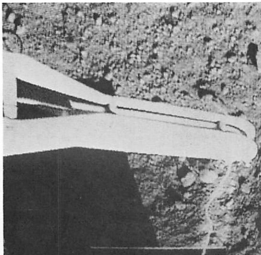
c) Inverse Fourier Transform of Gaussianly Quantized Fourier Transform of Boom, p = 500
