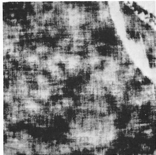
b) 10^{-1} Error Rate in the Fourier Domain
