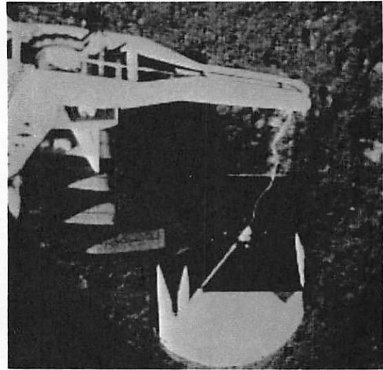
b) Inverse Fourier Transform of Fourier Transform
