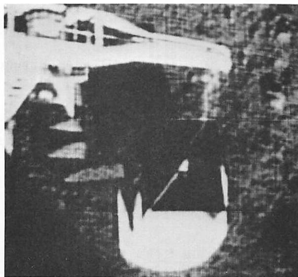
b) Fourier Transform of 300-level Thresholded Samples
