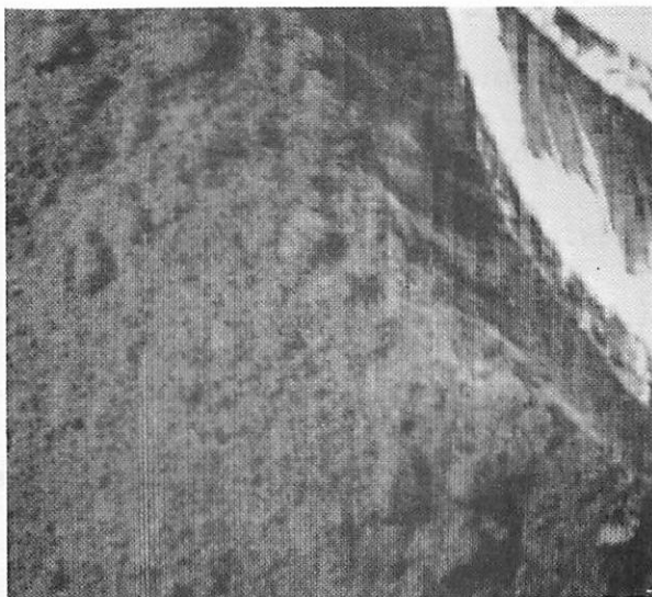
a) Hadamard Transform of Gaussianly Quantized Hadamard Transform with p = 500
