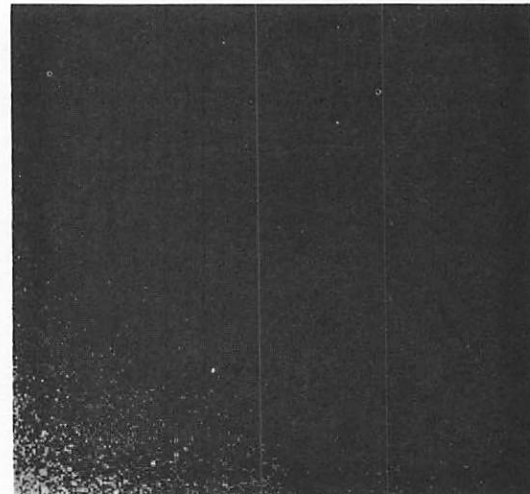
d) Logarithm of Magnitude of Hadamard Transform
