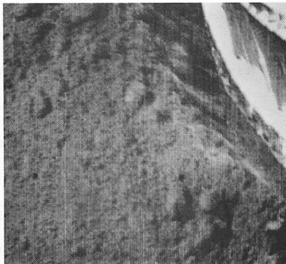
b) Hadamard Transform of Gaussianly Quantized Hadamard Transform with p = 1000
