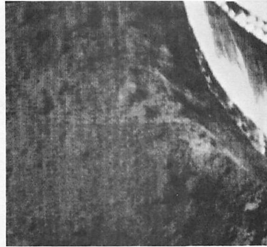
b) Inverse Fourier Transform of Gaussianly Quantized Fourier Transform of Footpad, p = 500
