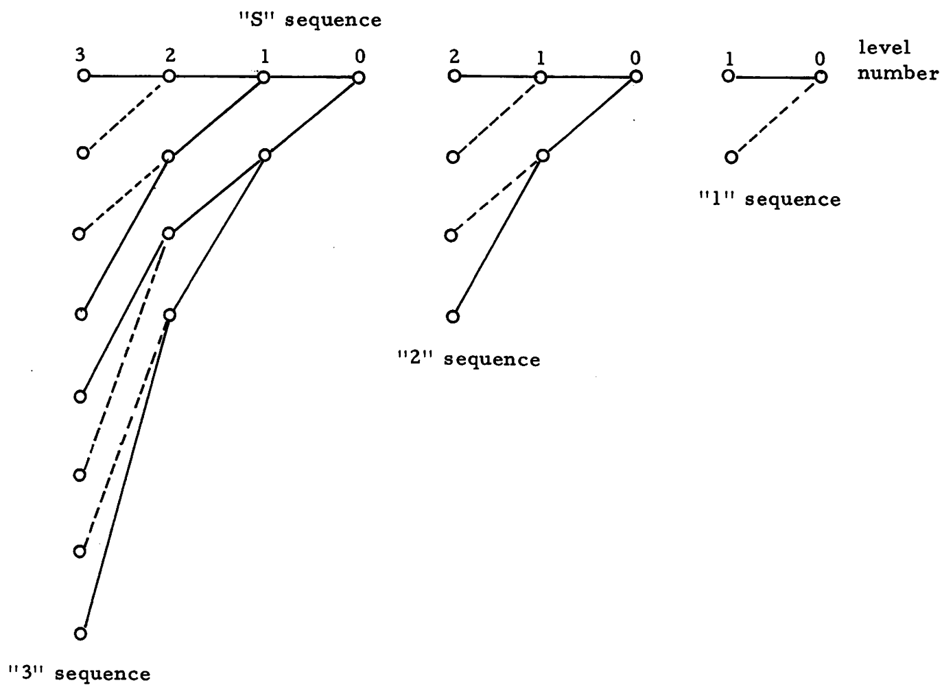
Figure A-2. Hadamard transform computational sequences.
