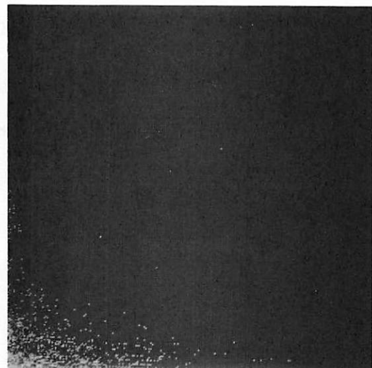
d) Logarithm of Magnitude of Hadamard Transform
