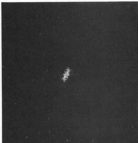
c) Magnitude of Fourier Transform
