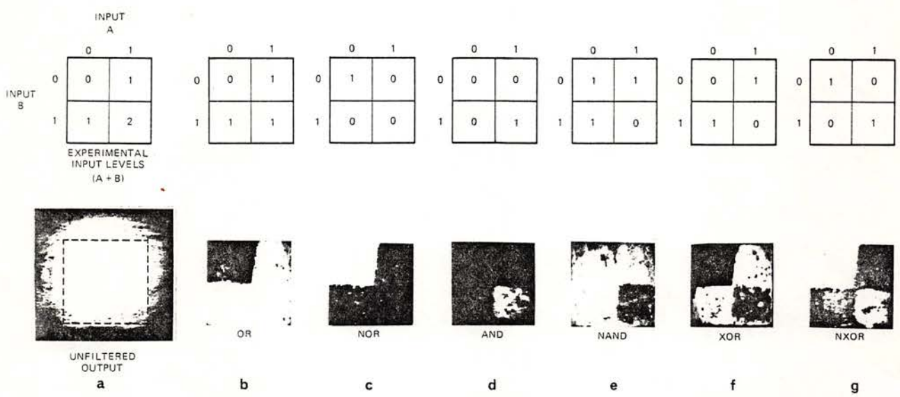
Figure 8. VGM logic results. (a) Two binary images were superimposed to produce the input intensities on the photoconductor as shown. Without any filter, the output is ideally a uniform field (logical 1). The actual output is shown below the indicated input levels. (b-g) indicate the ideal outputs and the actual outputs for the logical operations OR, NOR, AND, NAND, XOR, NXOR, respectively.
