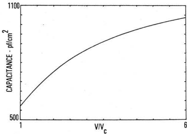
Figure 8. Cell capacitance vs. normalized voltage.
