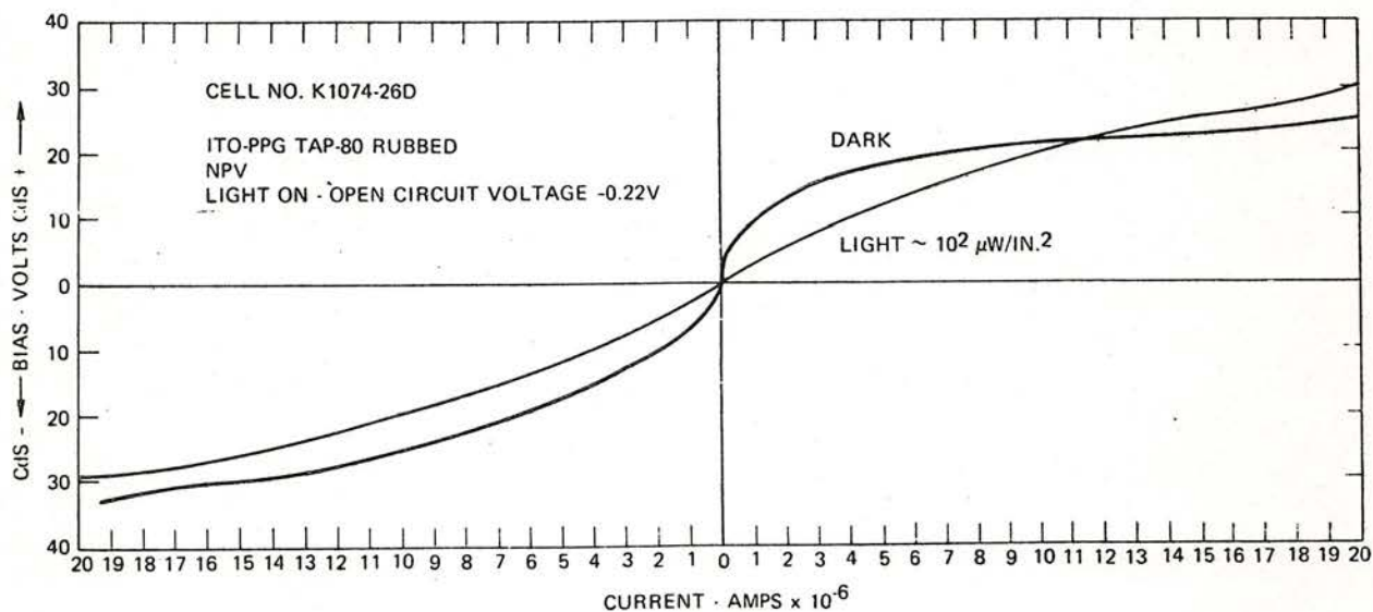
Figure 6. Junction effect in VGM cell.
