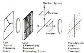
Fig. 2. System for parallel A/D conversion.
