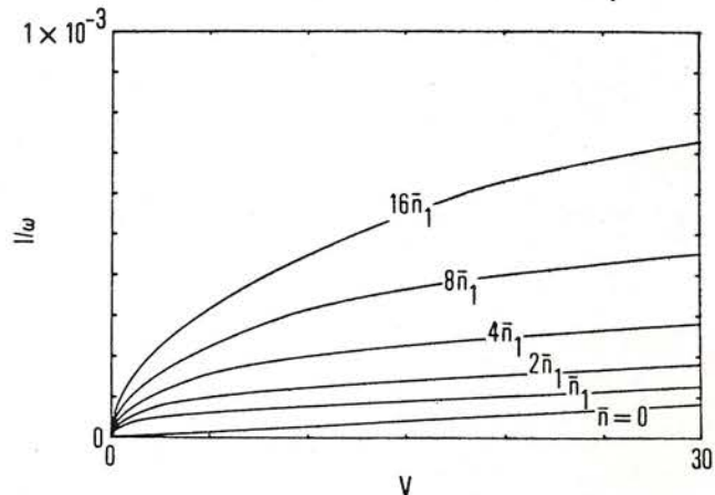
Figure 4. Normalized photosensor current vs. applied voltage.
