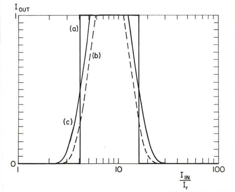
Figure 3. Level slice function for a piecewise linear model of a recording medium with \gamma = 3.0 . (a) Ideal. (b) Degraded. (c) Optimized.
