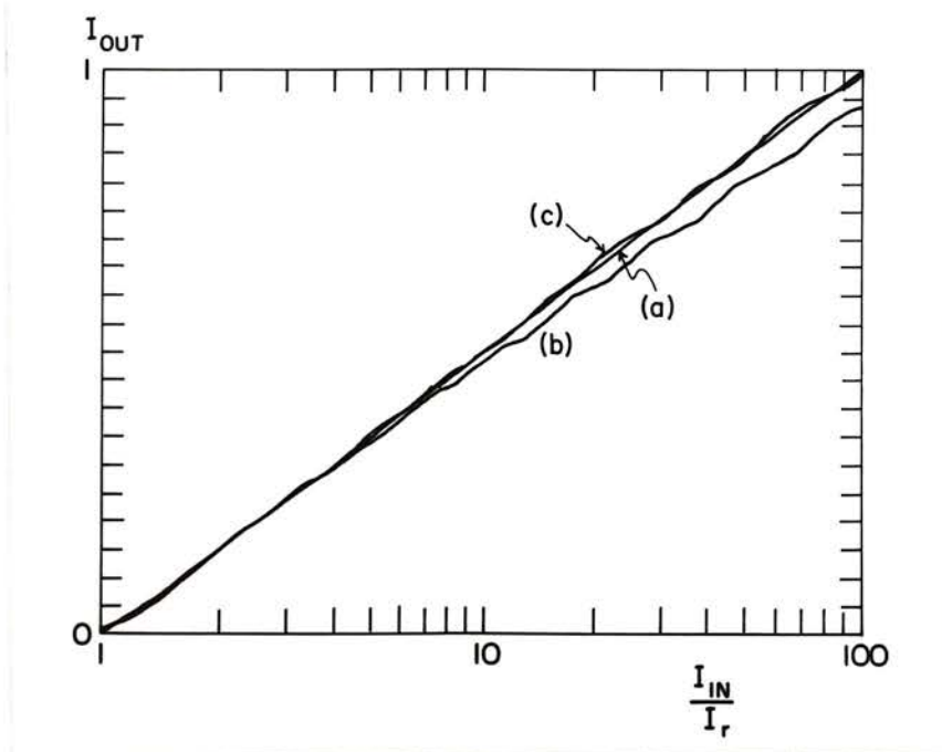
Figure 2. Logarithmic function for a piecewise linear model of a recording medium with \gamma = 3.0 . (a) Ideal. (b) Degraded. (c) Optimized.
