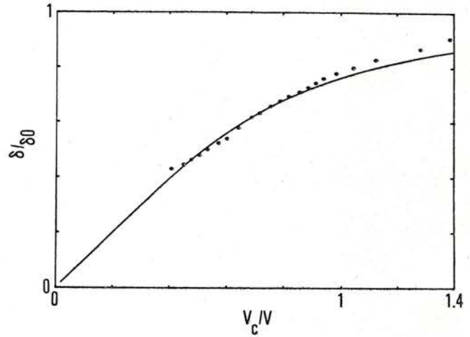
Figure 11. Measured phase retardation vs. inverse voltage.
