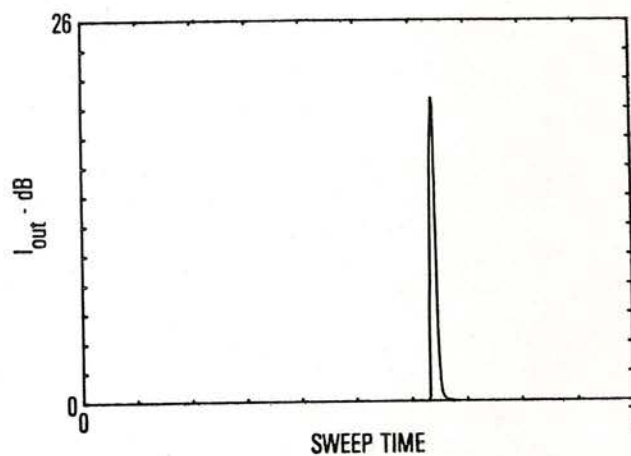
Figure 12. Preintegrated output response for level slice operation
