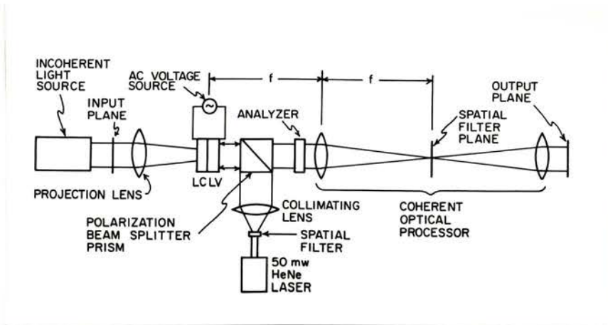
Figure 5. Experimental setup for real-time halftone processing with a LCLV.
