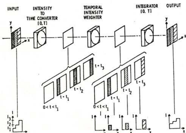
Figure 1. Operation of nonlinear image processor
