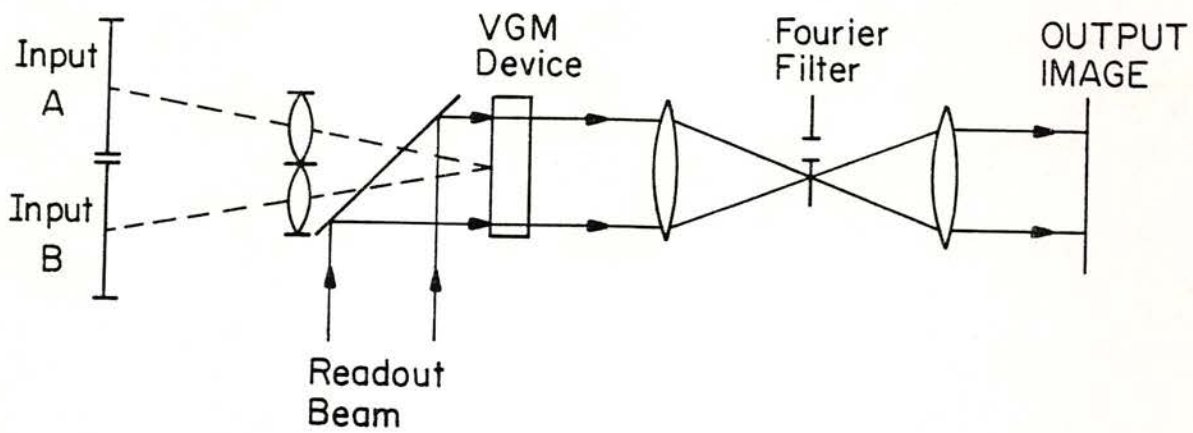
Figure 7. Experimental arrangement for performing logical operations on two dimensional binary inputs with a VGM device. The two input images are superimposed on the photoconductor. The device is read out in transmission. Simple slit apertures can be used to achieve the desired logic operations.
