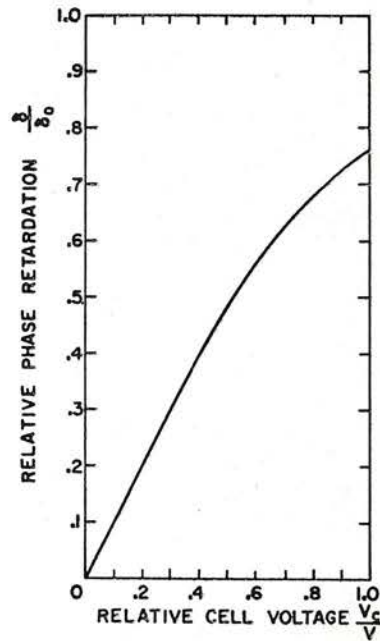
Figure 7. Normalized phase retardation vs. inverse normalized voltage.
