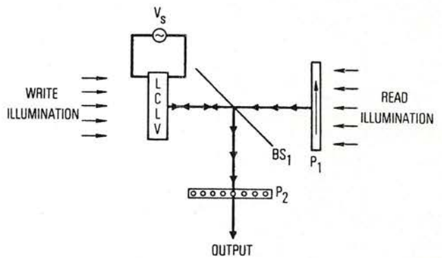
Figure 9. Test configuration for measuring response of LCLV.
