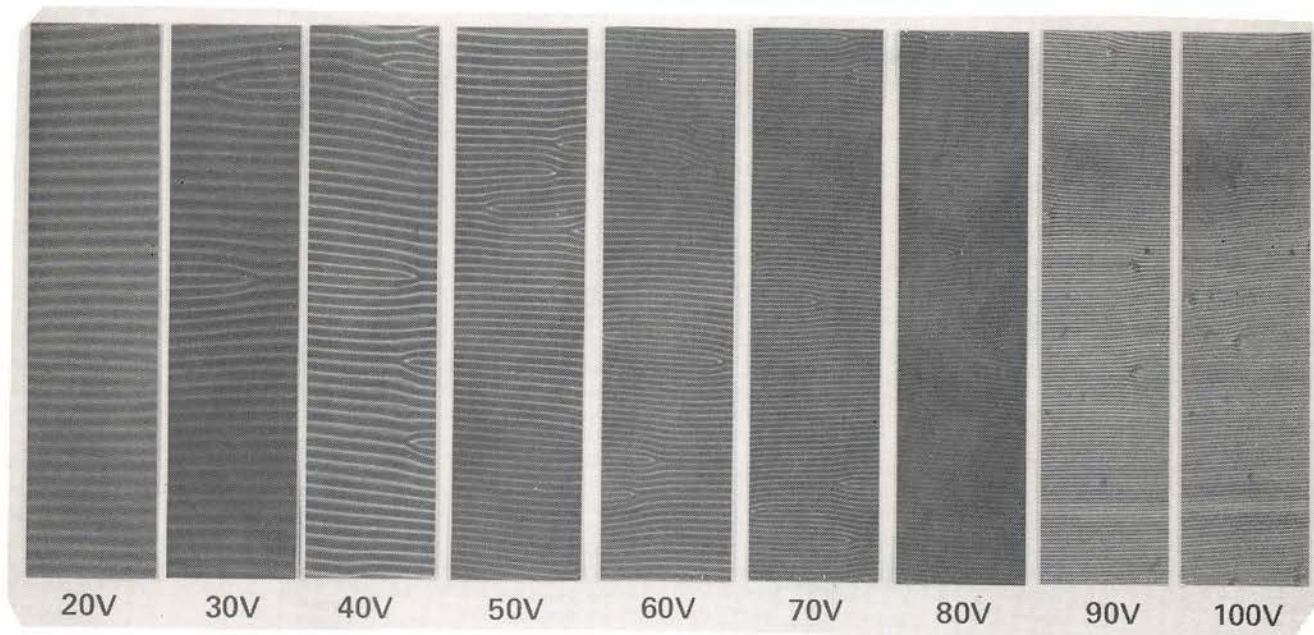
Figure 1. VGM viewed through polarizing microscope.
