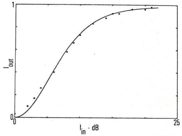
Figure 13. Measured and calculated response of LCLV.
