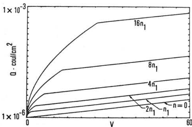
Figure 3. Q vs. V curves for CdS/CdTe photosensor.
