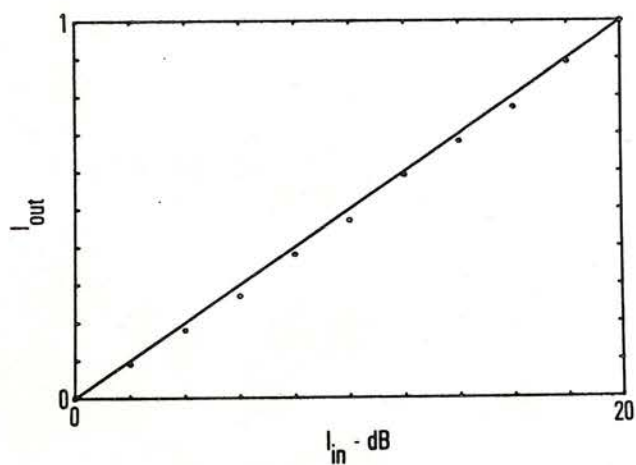
Figure 13. Logarithm operation response
