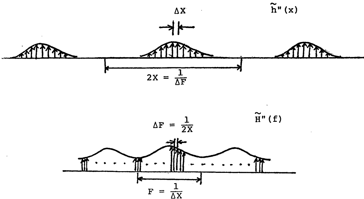
Figure 7. Fourier transform pair \tilde{h}''(x) \Leftrightarrow \tilde{H}''(f) where \tilde{H}(f) is sampled finer. ( M=2 )
