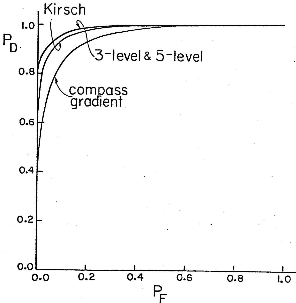
(b) template operators, SNR=10
